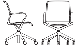
9421PA Conference Chair—Mesh Back, Upholstered Seat, Polished Aluminum Base W 25.5" D 26" H 35.5–40.5" SH 19–24" AH 26–31"
