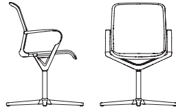
9461PA Guest Chair—Mesh Back, Upholstered Seat, Polished Aluminum Base W 26.5" D 26.5" H 35" SH 18.5" AH 25"
