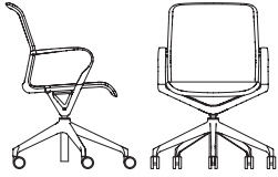
9411PA Conference Chair—Polished Aluminum Base W 25.5" D 26" H 35.5–40.5" SH 18.5–23.5" AH 26–31"
